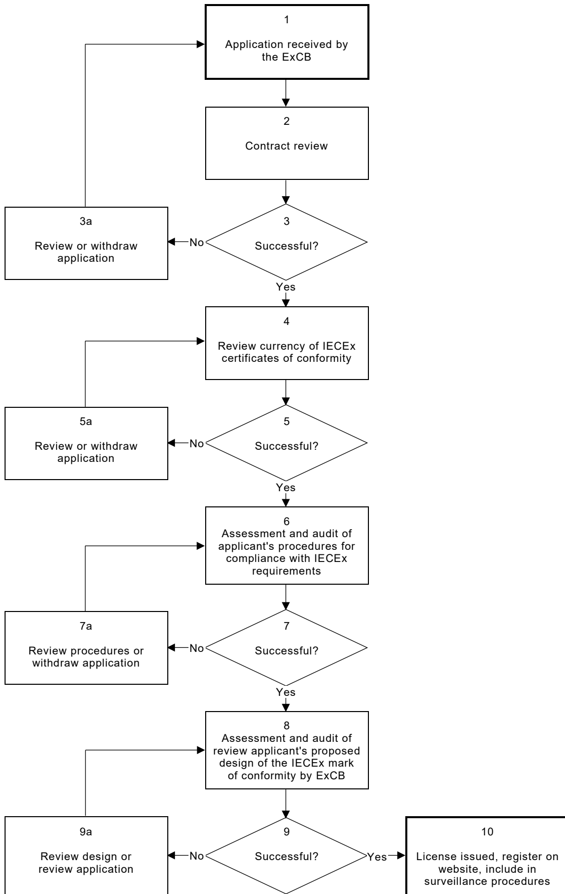
Figure 2 – Overview of ExCB process to issue IECEX conformity mark license
